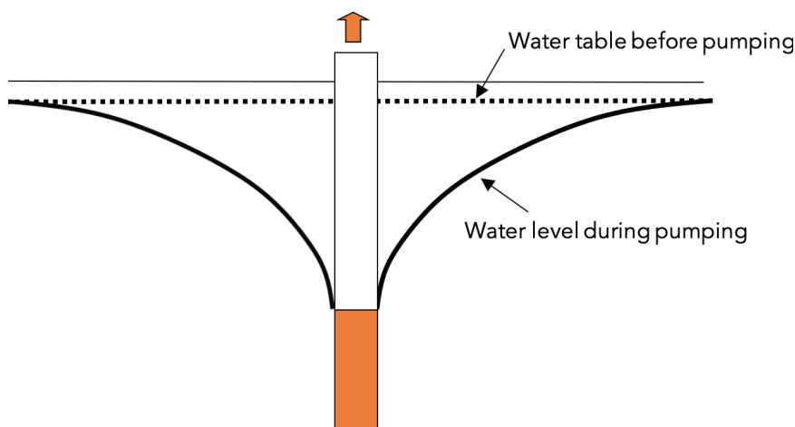
Figure 3.10 The cone of depression or drawdown curve around a well or borehole
