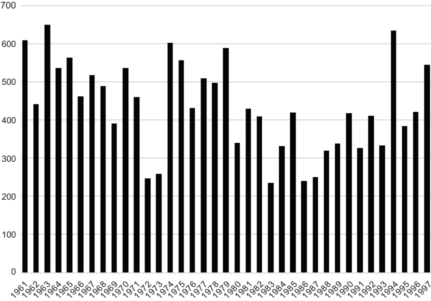
Nguru, north-east Nigeria, a semi-arid location. Mean annual rainfall 436 mm, CV 27%
