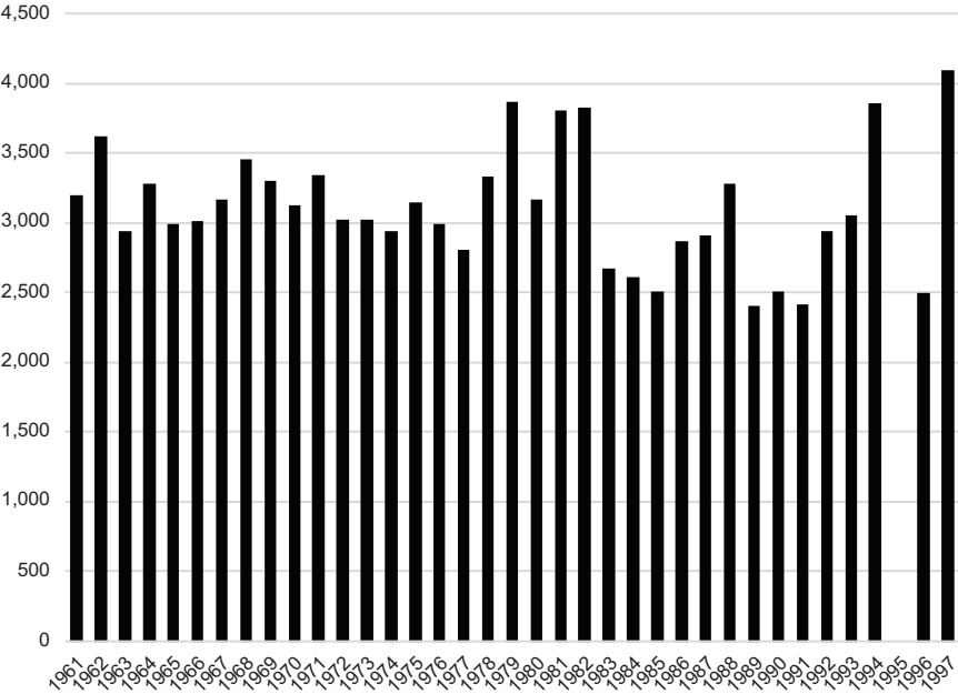
Makeni, northern Sierra Leone, with a tropical monsoon climate. Mean annual rainfall 3,111 mm, CV 14%
