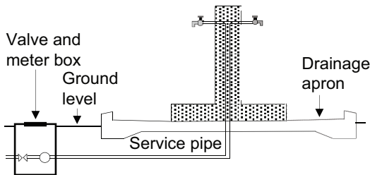
Figure 6.1 Simple branched gravity flow schemes
