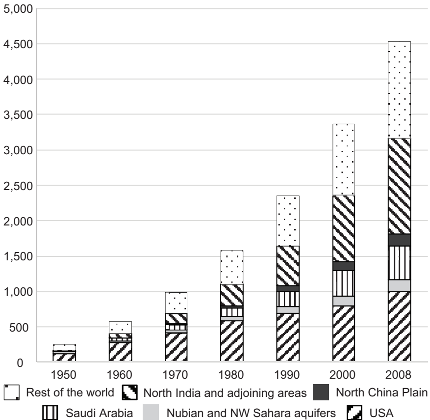
Figure 3.6 Estimated cumulative groundwater depletion by region since 1900, km 3
