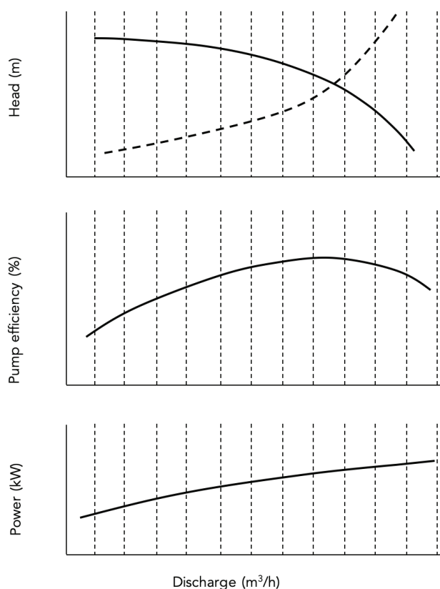
Figure 6.4 Submersible pump characteristic curves
