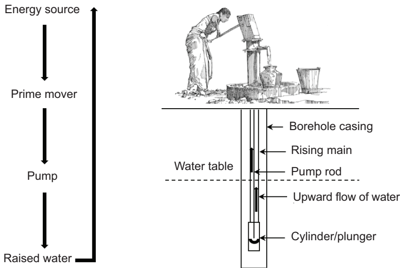
Figure 5.1 Water pump components, conceptually and practically Note: The energy source is food; the prime mover is the pump operator; the pumping element is the submerged cylinder and plunger; power is conveyed to the plunger via the pump rods, with or without a lever Source: Sketch courtesy of Rod Shaw (2015), WEDC, Loughborough University
